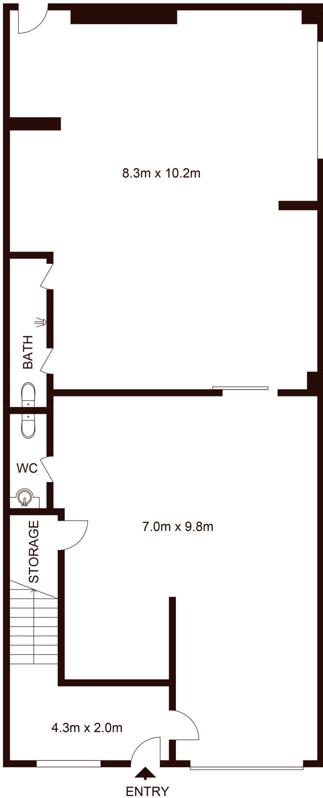
GROUND FLOOR
