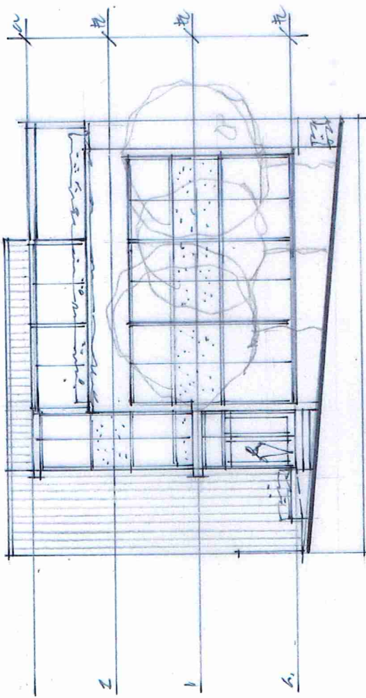
ELEVATION - HAYNES ST
