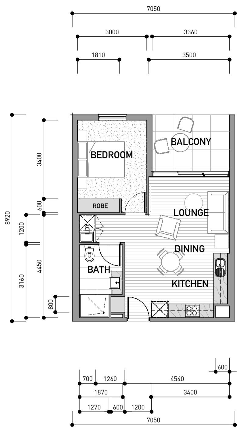
APARTMENT - 1 BEDROOM TYPE (INC BALCONY) [46.70 + 9.4] - 56.10 SQM
