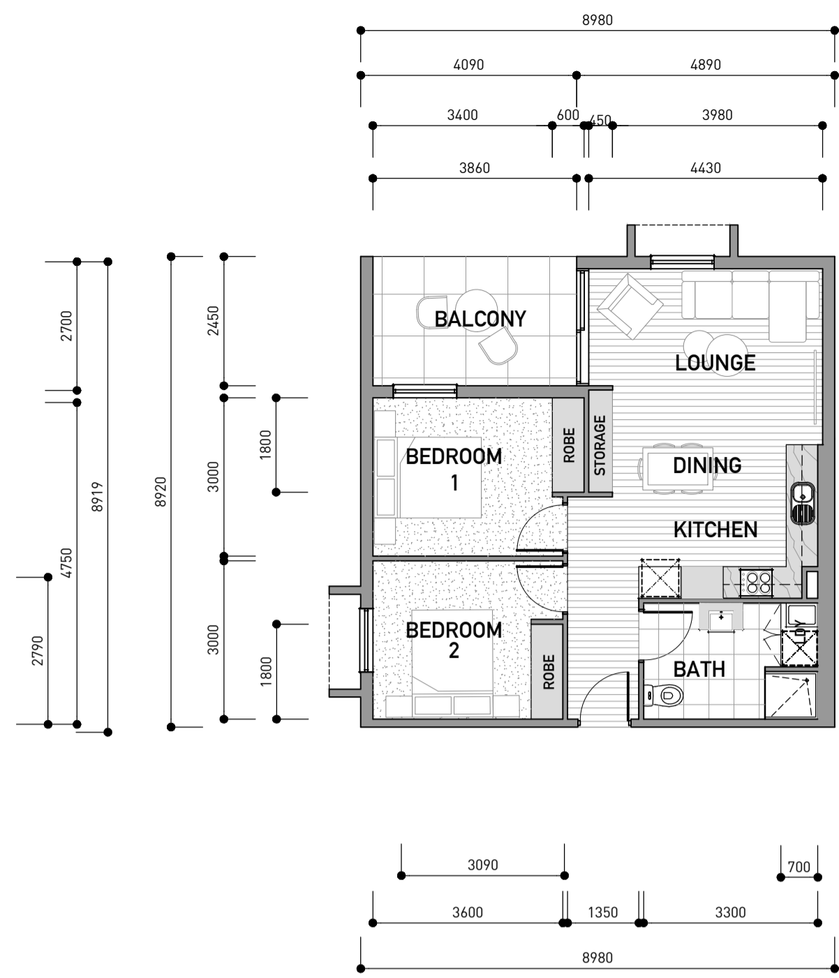
APARTMENT 2 BEDROOM TYPE (INC BALCONY) [66.03+11] - 76.03SQM
