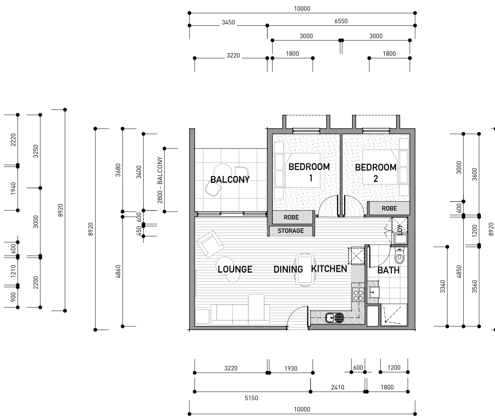
APARTMENT 2 BEDROOM TYPE (INC BALCONY) [63.88 + 11] - 73.88 SQM
