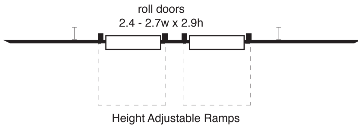
Plan View
