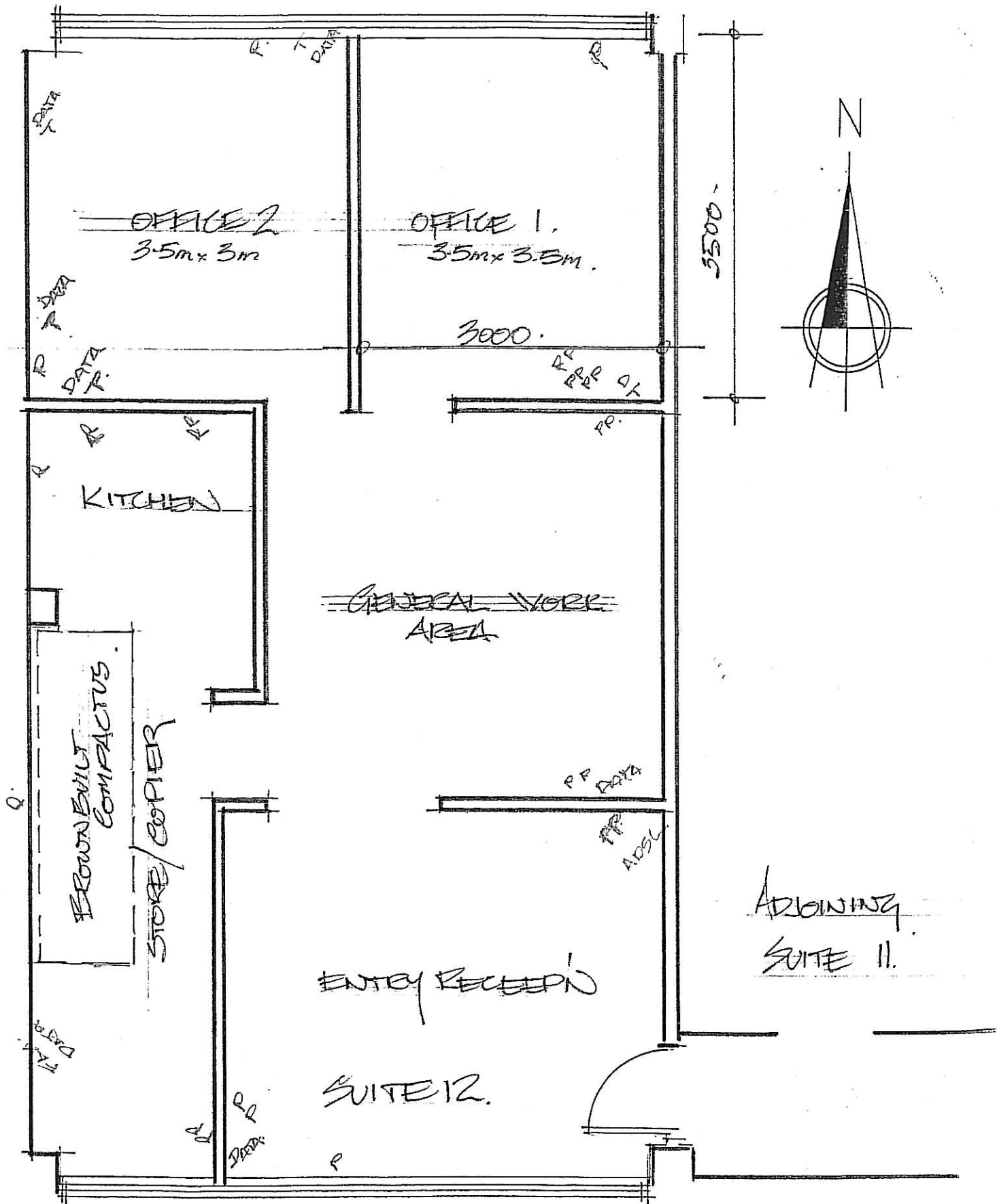
○ FLOOR PLAN 1:50
