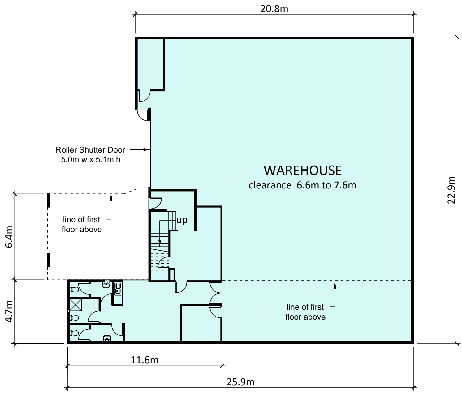
GROUND FLOOR
