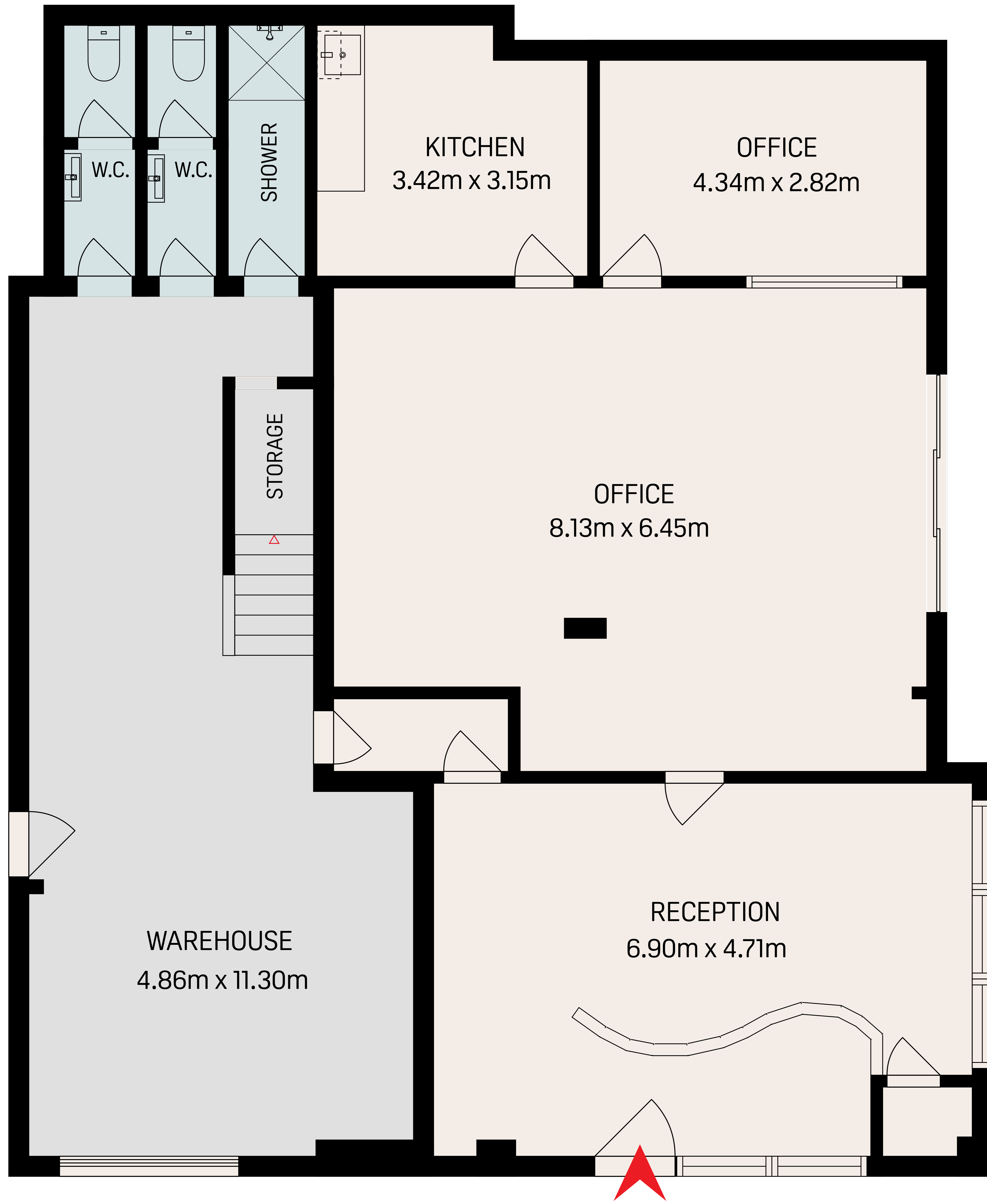
FLOOR 1
