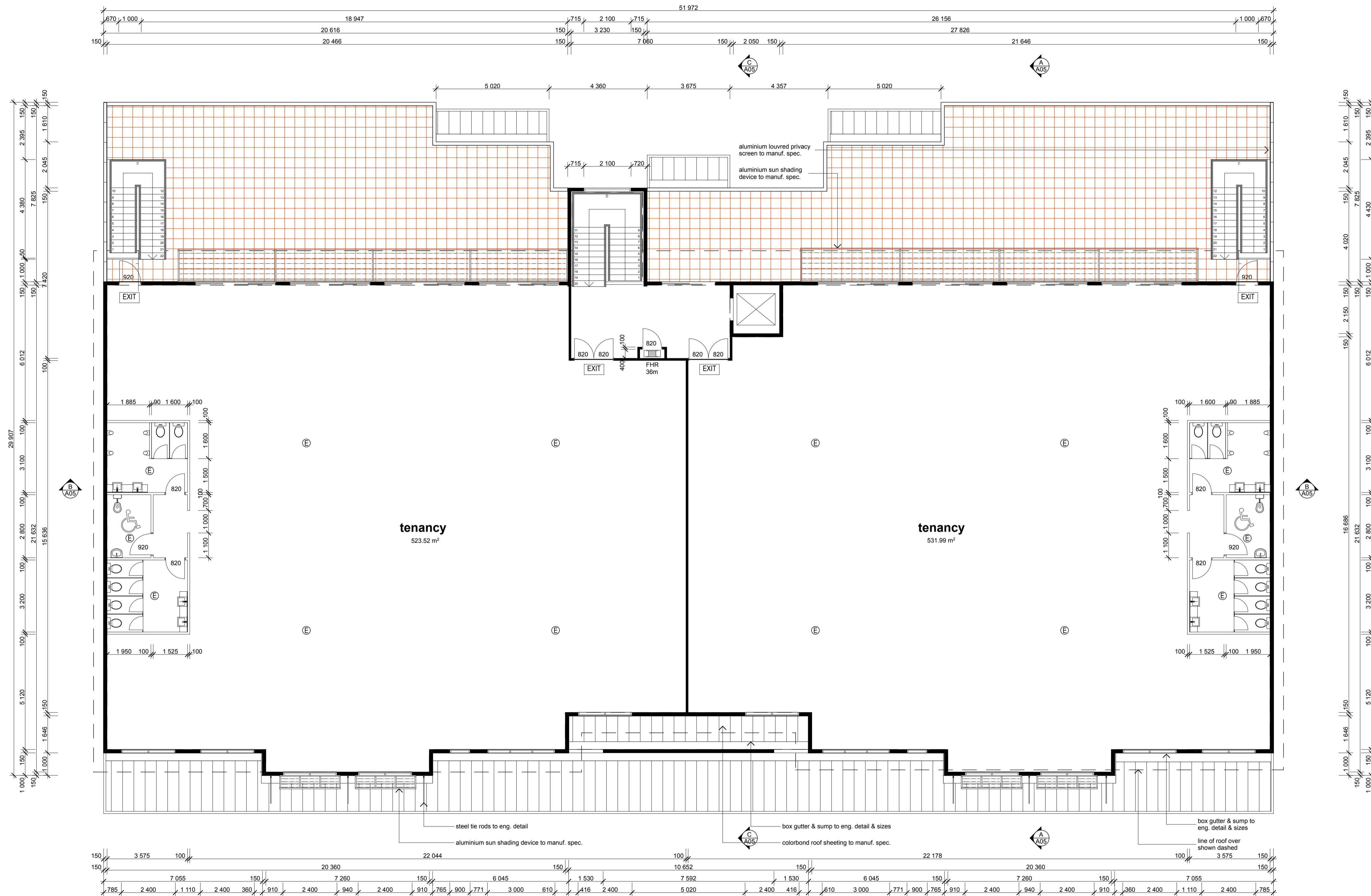
Level 1 Floor Plan 1:100
