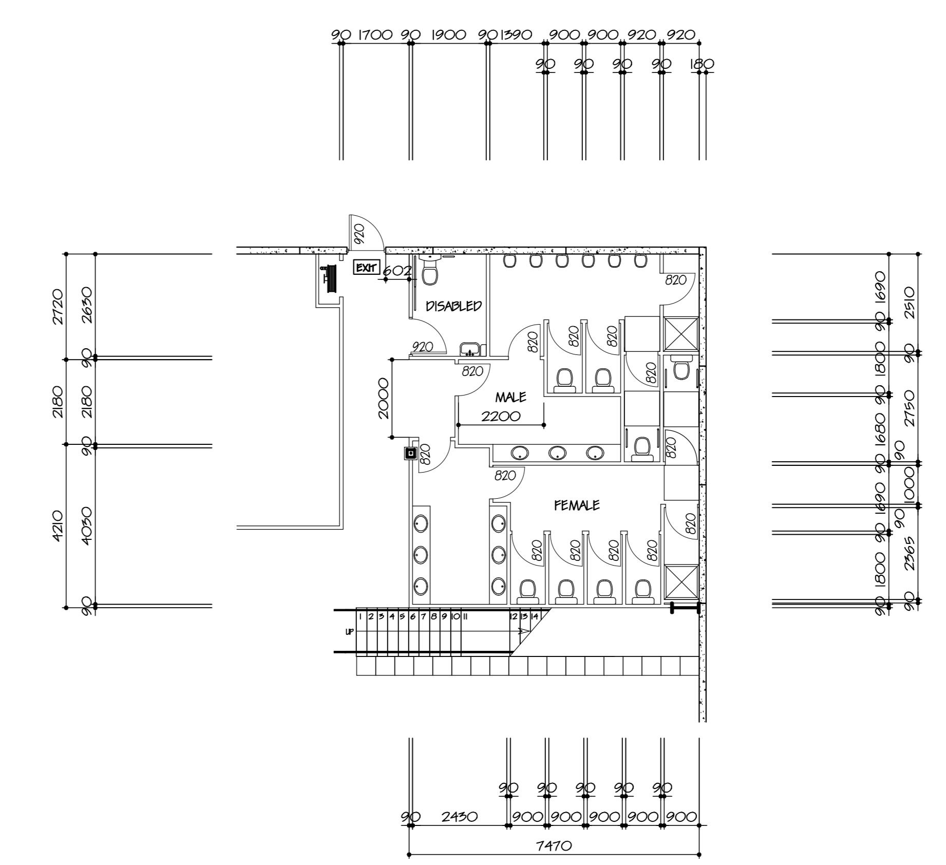
GROUND FLOOR AMENITY LAYOUT
