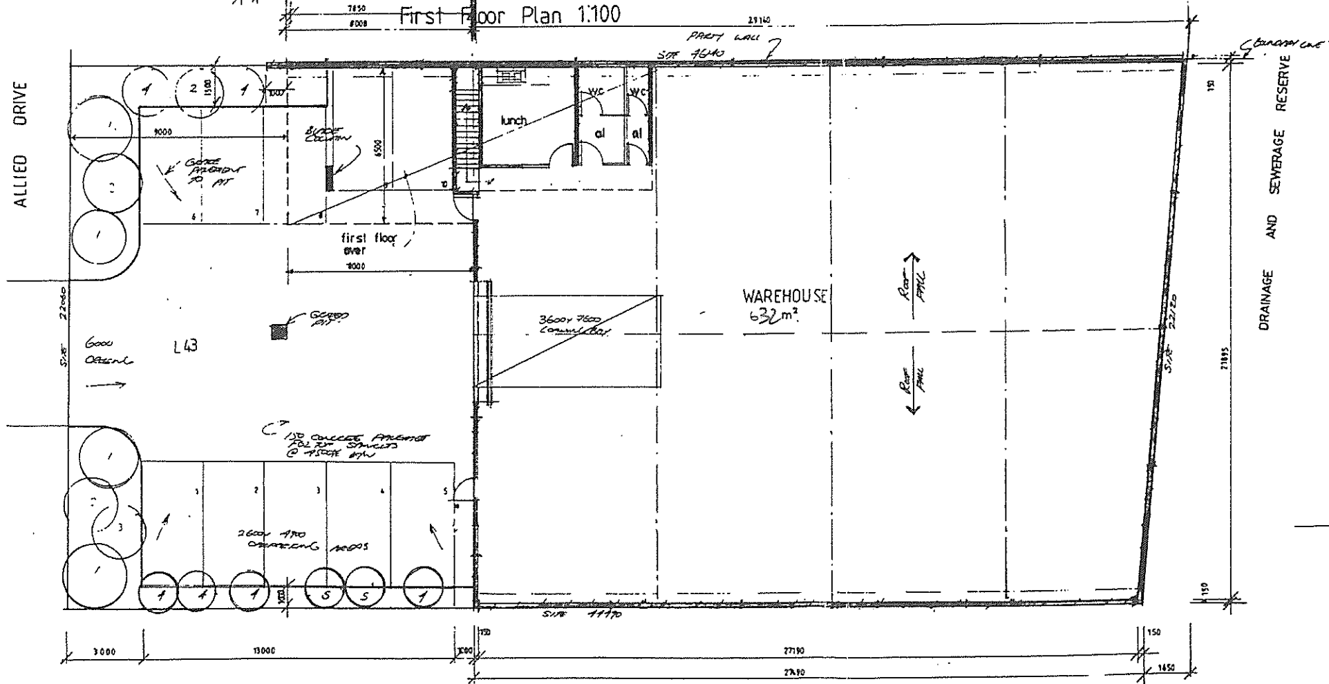
Site / Ground Floor Plan 1:100
