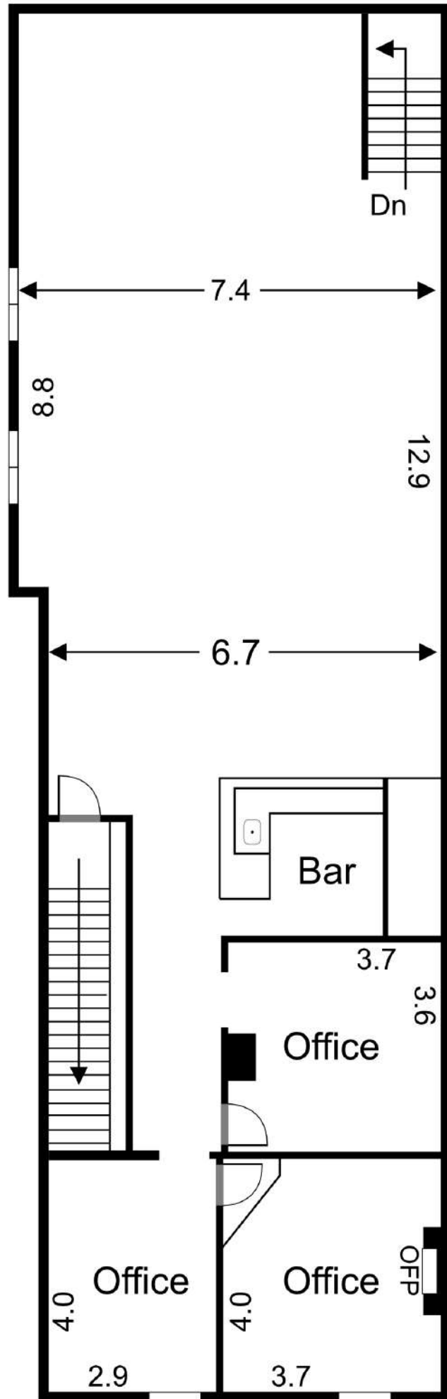
FIRST FLOOR
