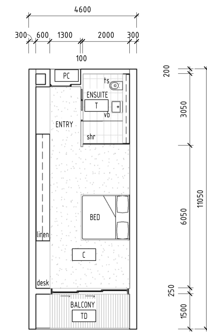
2 TYPICAL HOTEL ROOM PLAN TP02 1 : 100
