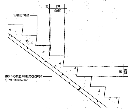
RISE AND GOING DETAIL (TYP) SCALE 1:20
