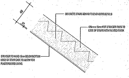
STRINGER DETAIL (TYP) SCALE 1:20
