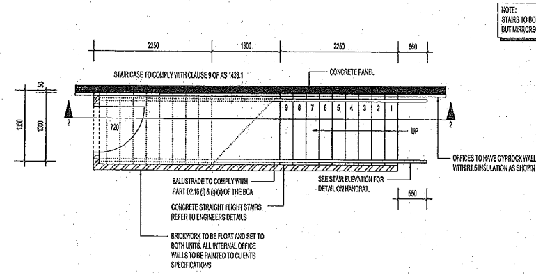
UNIT 1 2-2 PLAN STAIR DETAIL - GROUND FLOOR A03 SCALE 1:50
