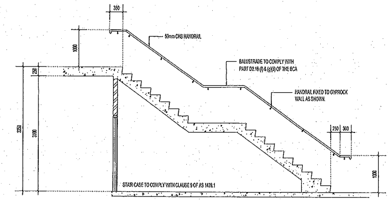
UNIT 1 2-2 STAIR SECTION 1 A03 SCALE 1:50
