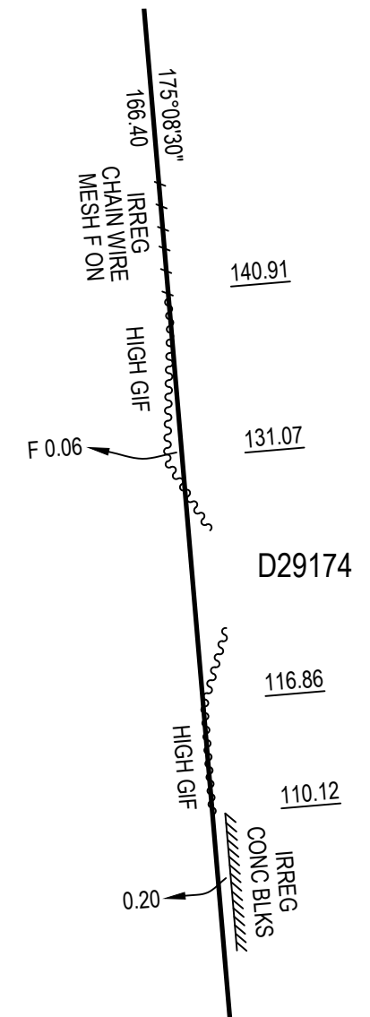
ENLARGEMENT C4 NOT TO SCALE
