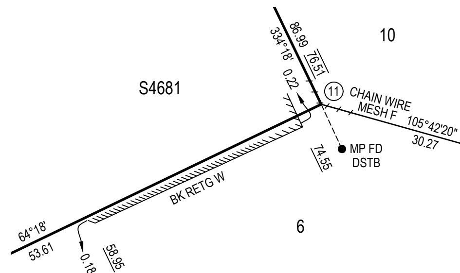
ENLARGEMENT B4 NOT TO SCALE
