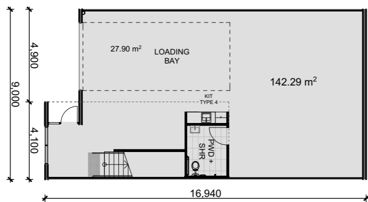
GROUND FLOOR PLAN 1:200 @ A3
