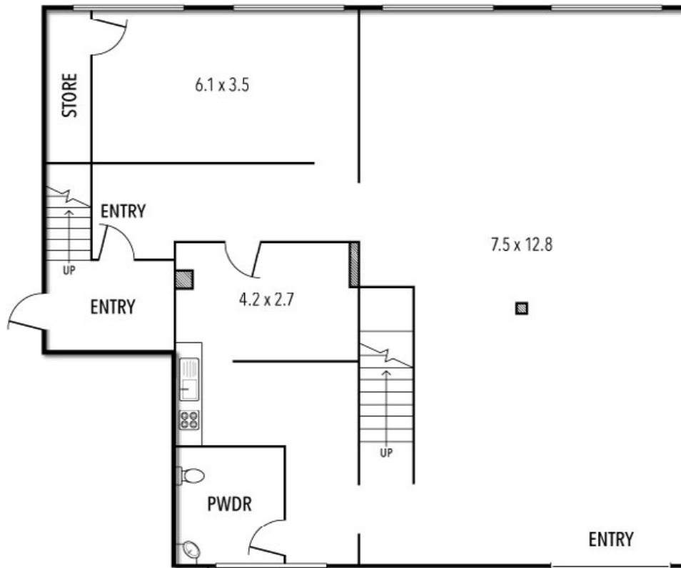
GROUND FLOOR
