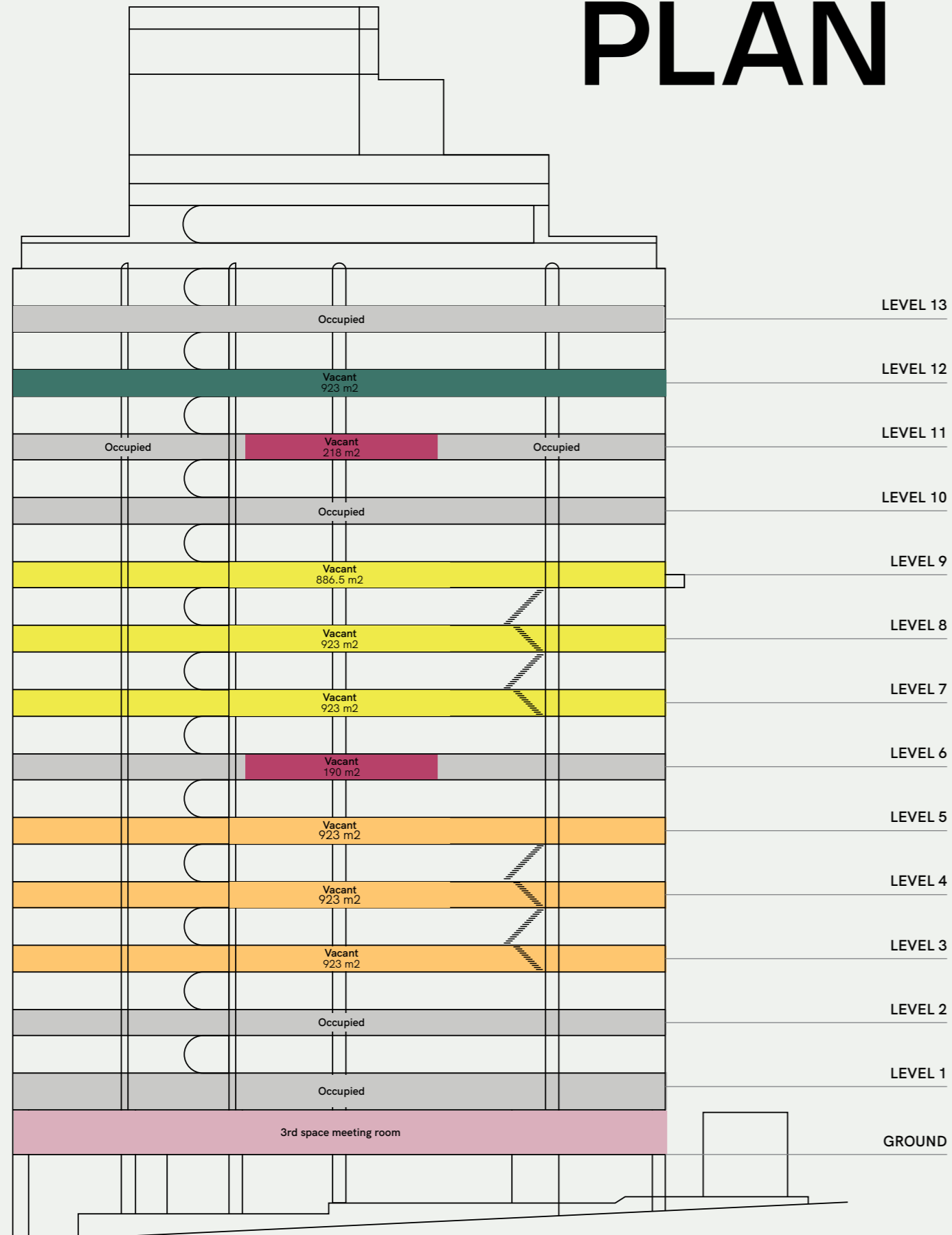
TOWER 1
