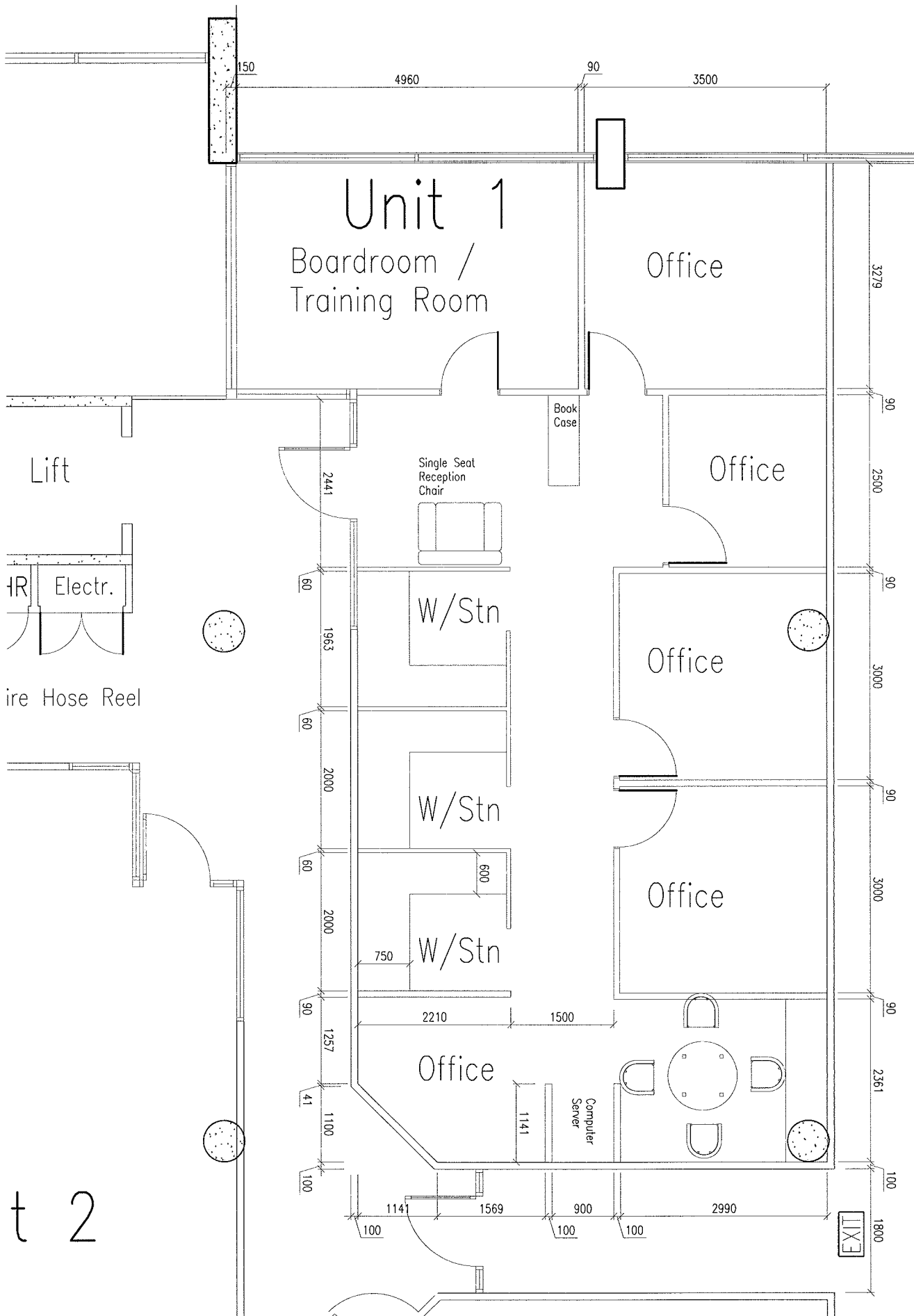
UNIT 1 - 1st FLOOR LAYOUT
