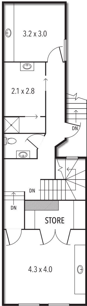
FIRST FLOOR
