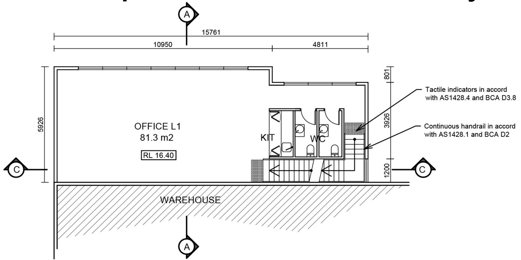
OFFICE FLOOR PLAN LEVEL 1
