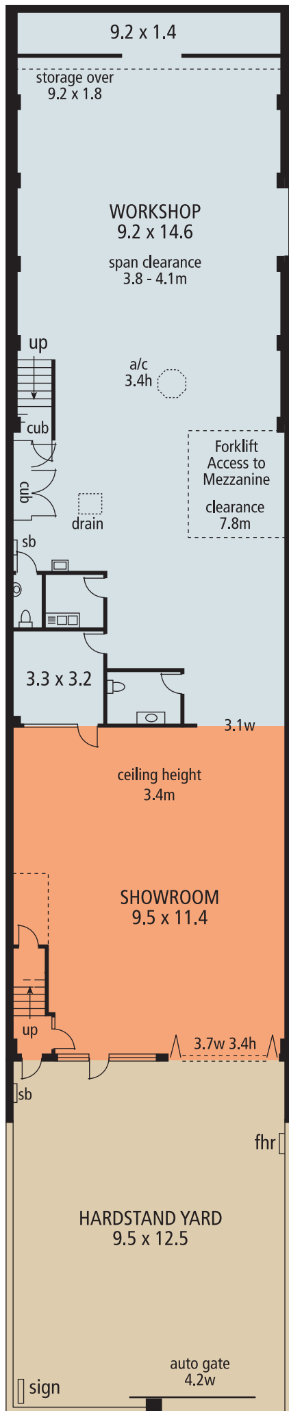
GROUND FLOOR
