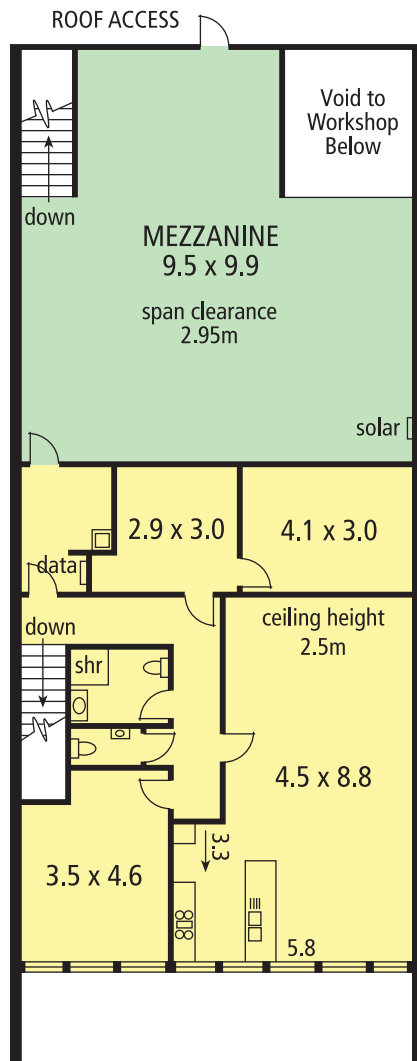
FIRST FLOOR
