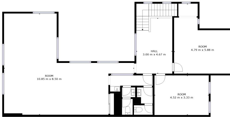
FLOOR 2
