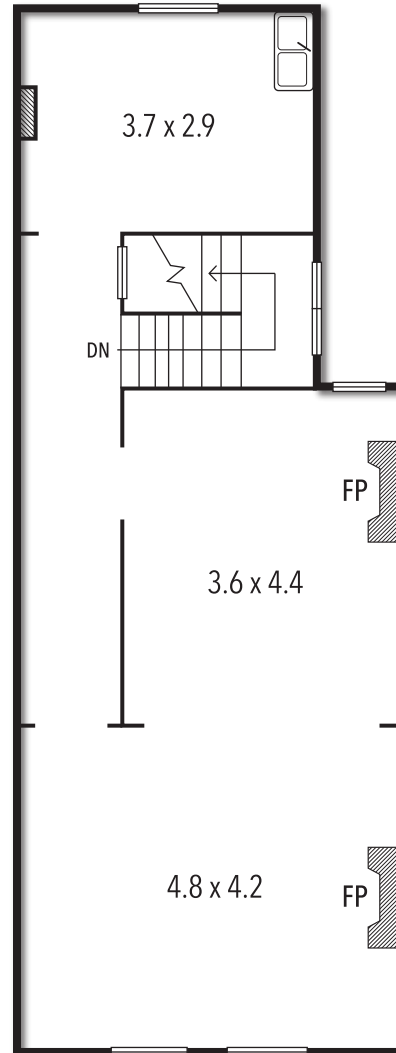
FIRST FLOOR
