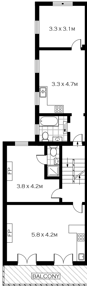
FIRST FLOOR
