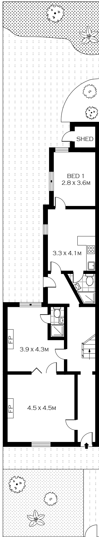
GROUND FLOOR
