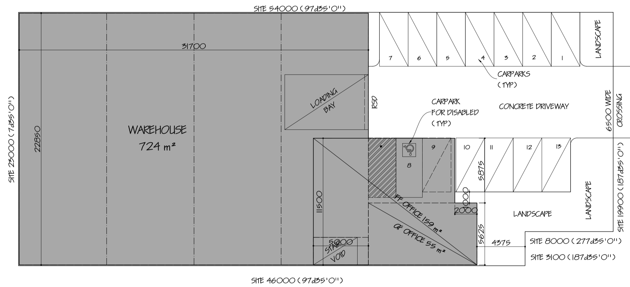
SITE DEVELOPMENT PLAN SKETCH 2
