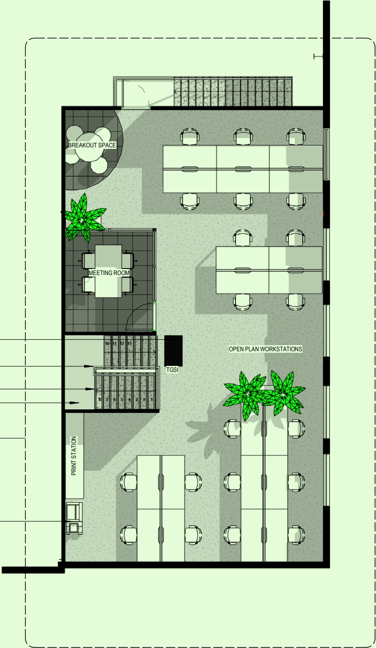
1 PROPOSED LEVEL 1 1:100
