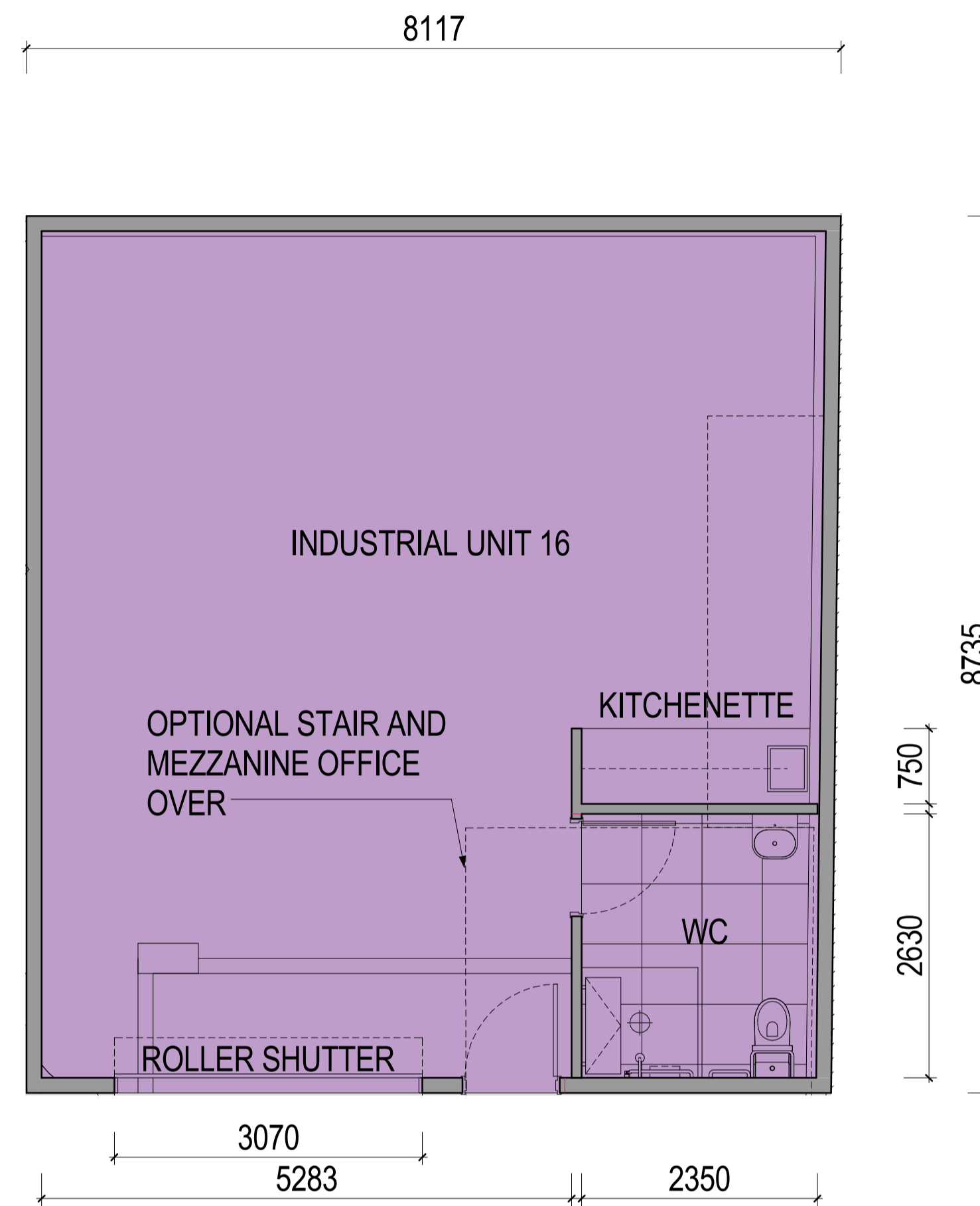
1 INDUSTRIAL UNIT 16 A03.01 SCALE 1:50
