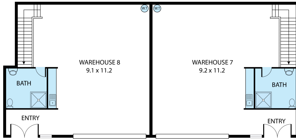
GROUND FLOOR
