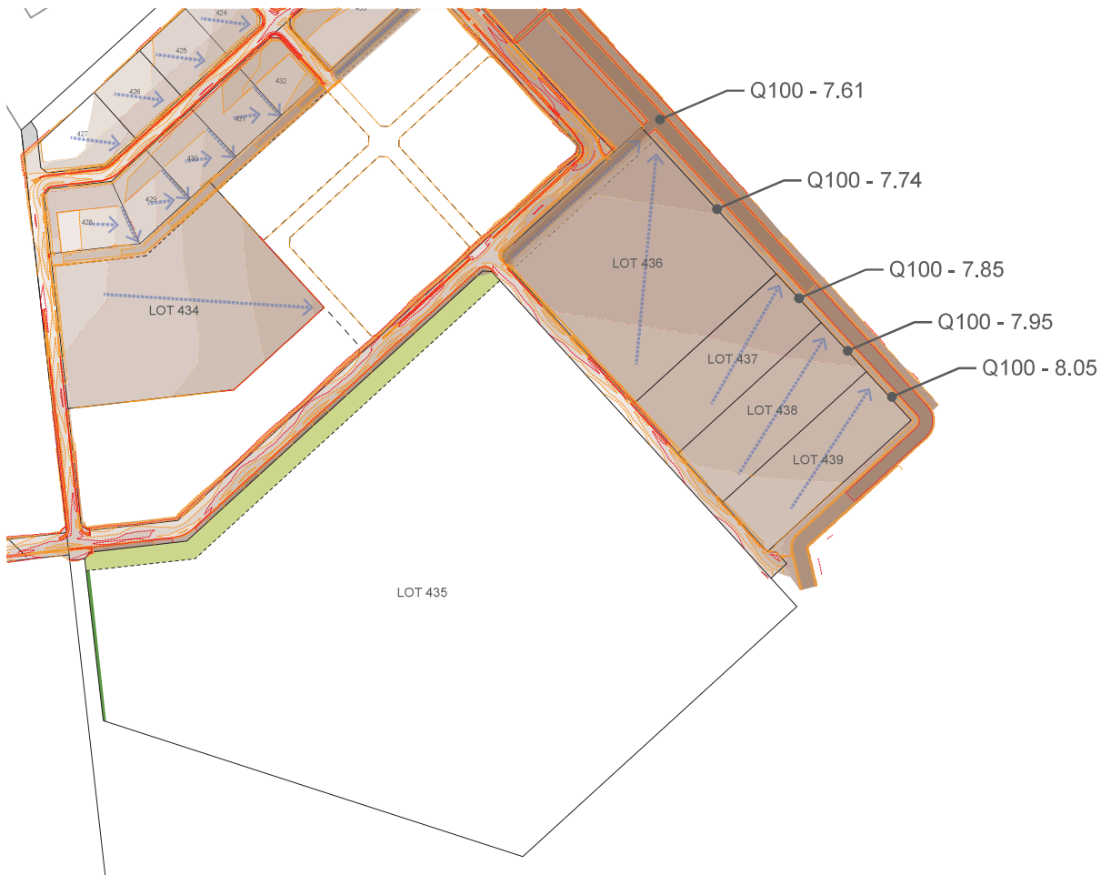
Figure 7.1a - Drainage Plan.
