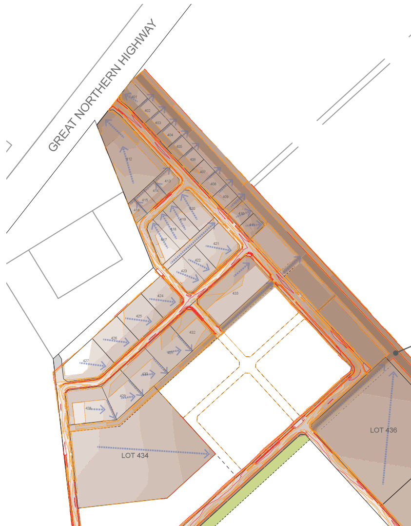
Figure 6.1a - Drainage Plan.
