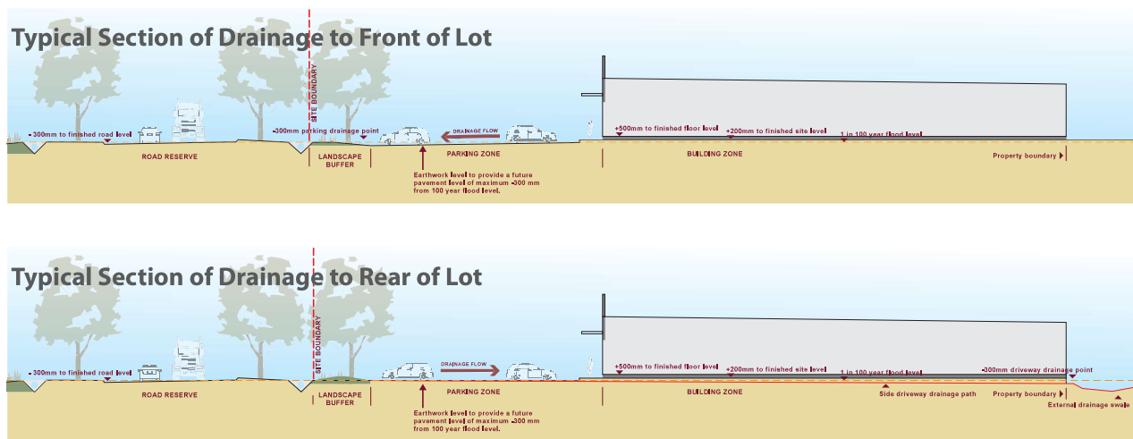
Figure 6.1b - Typical Sections through Different Lot Drainage Types
