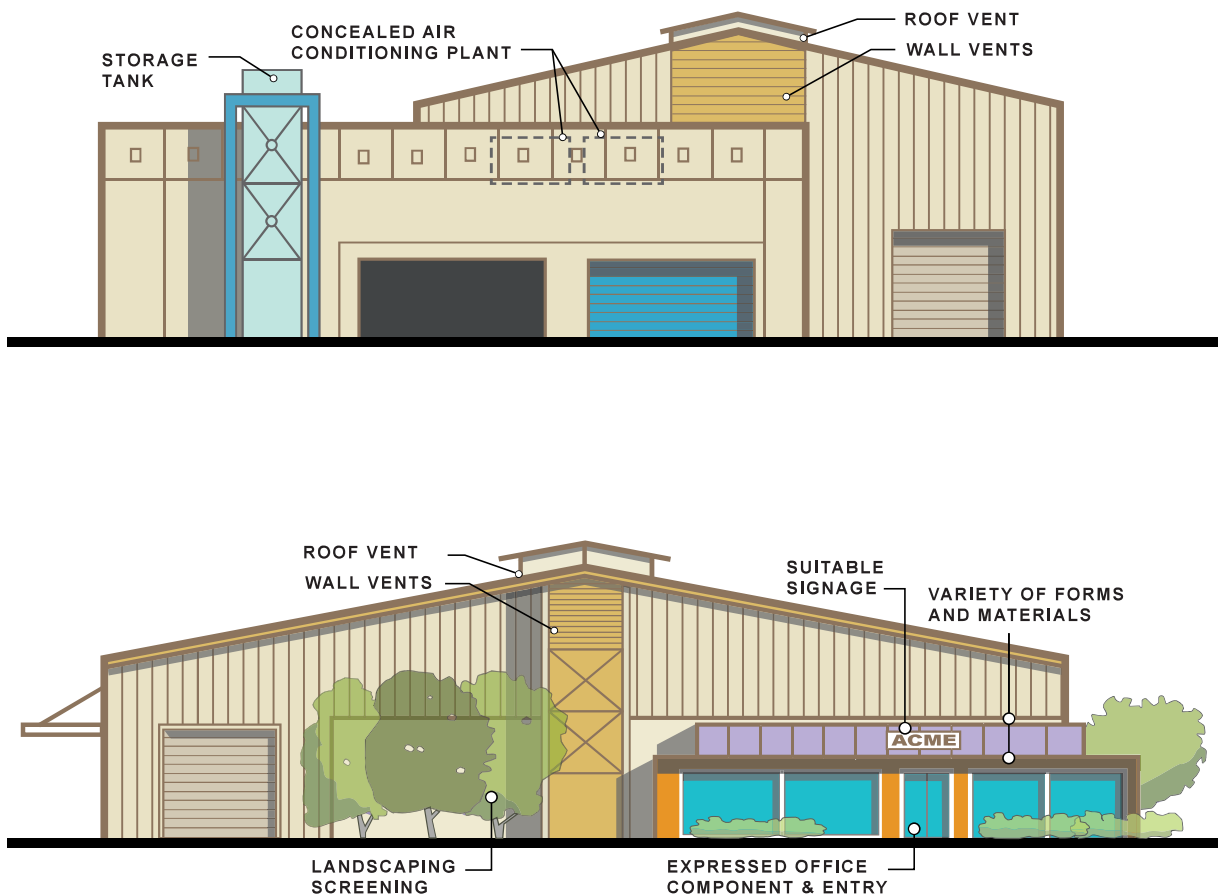
Figure 5.5a - Potential opportunities for integrating essential elements into the building design.
