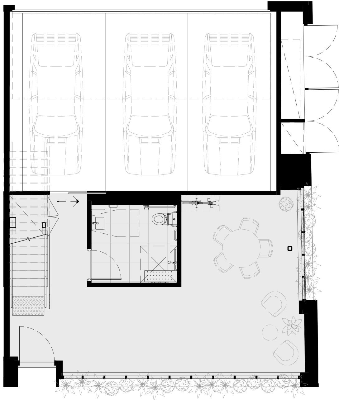
Ground Floor
