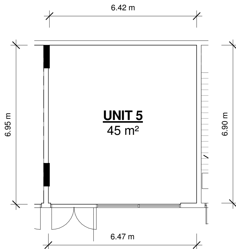
RETAIL UNIT 5 (GROUND FLOOR) 1 : 100
