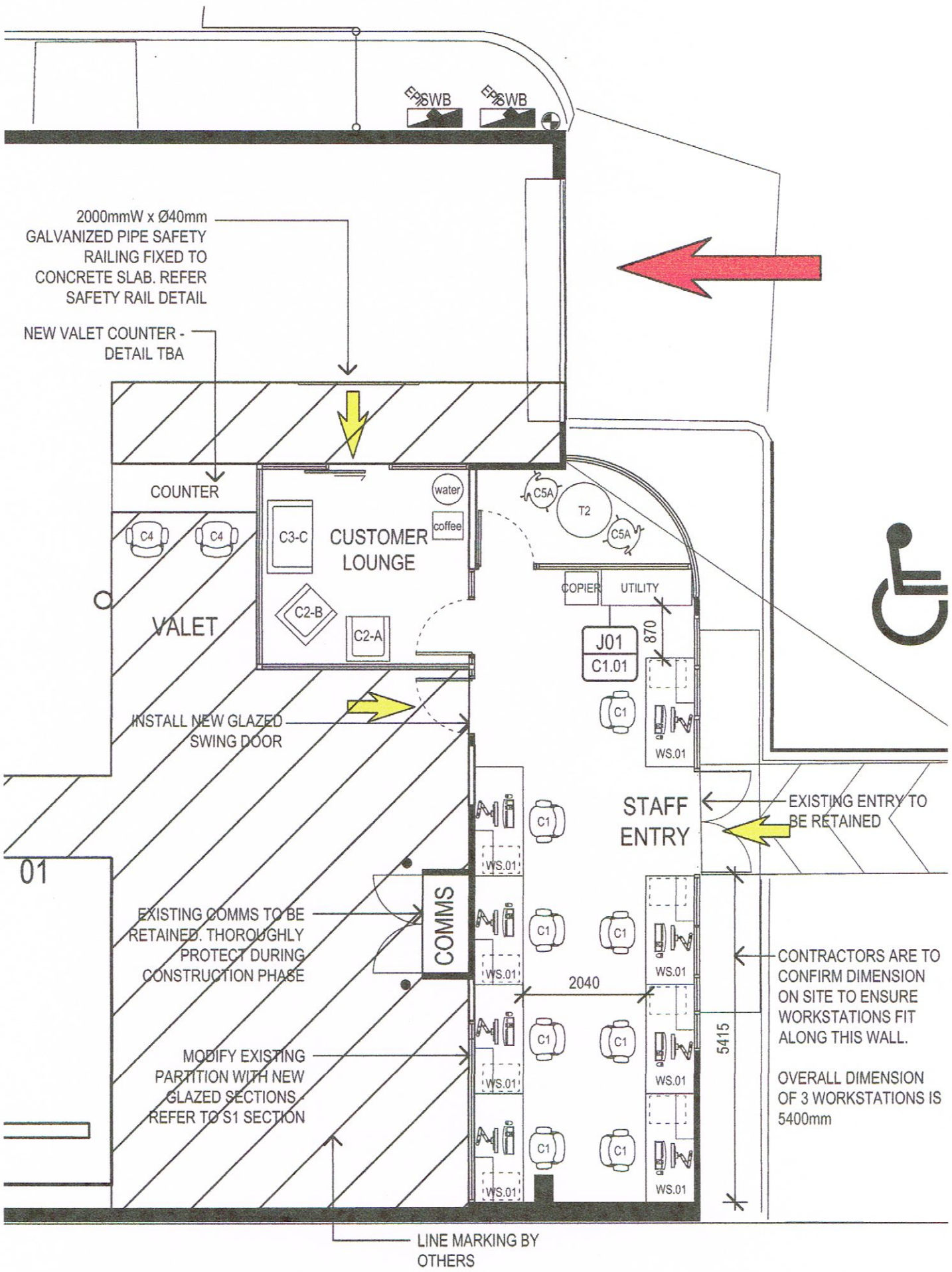
- Ground Floor Plan - Office Area - 1:100
