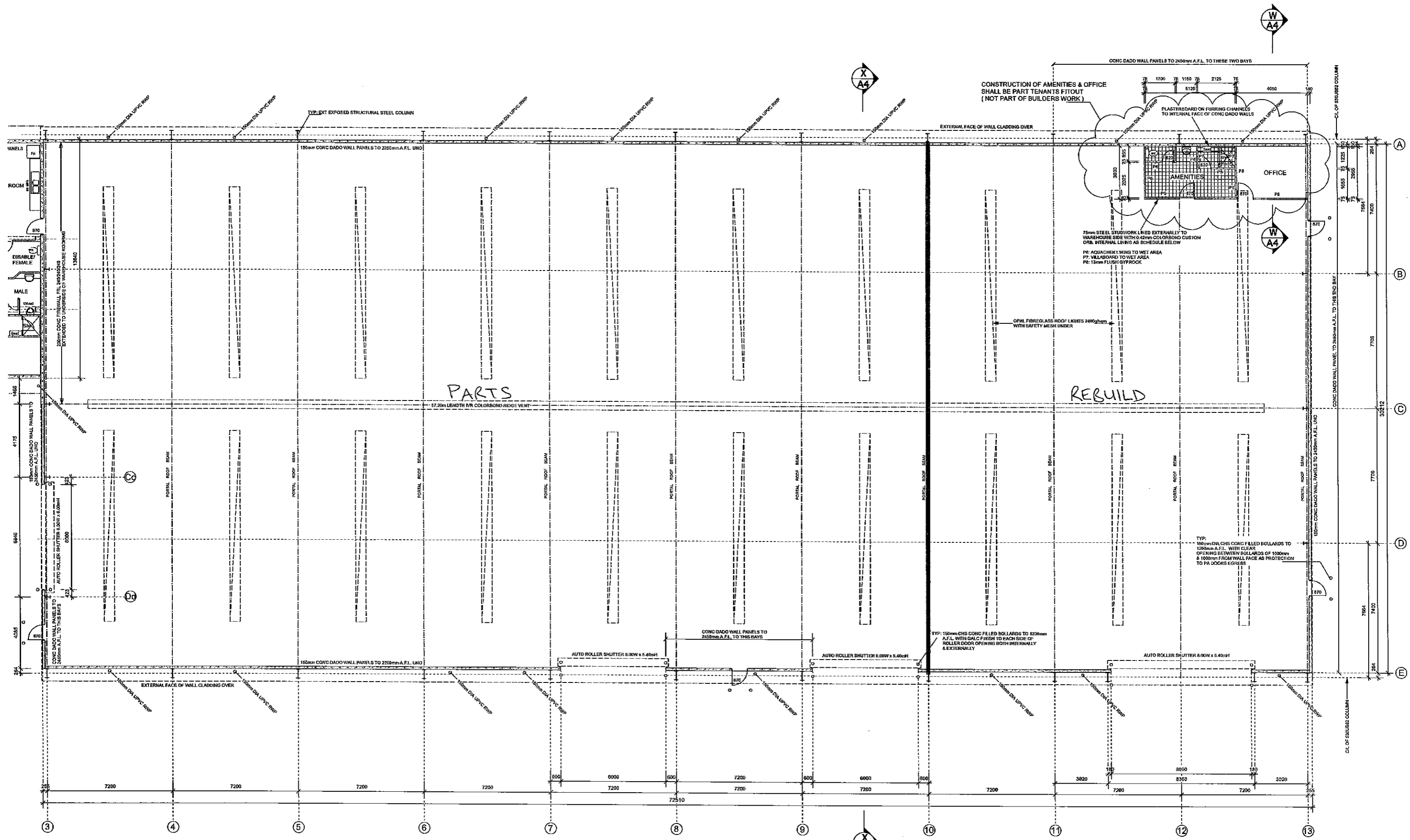
WAREHOUSE / WORKSHOP GROUND FLOOR PLAN 1:100
