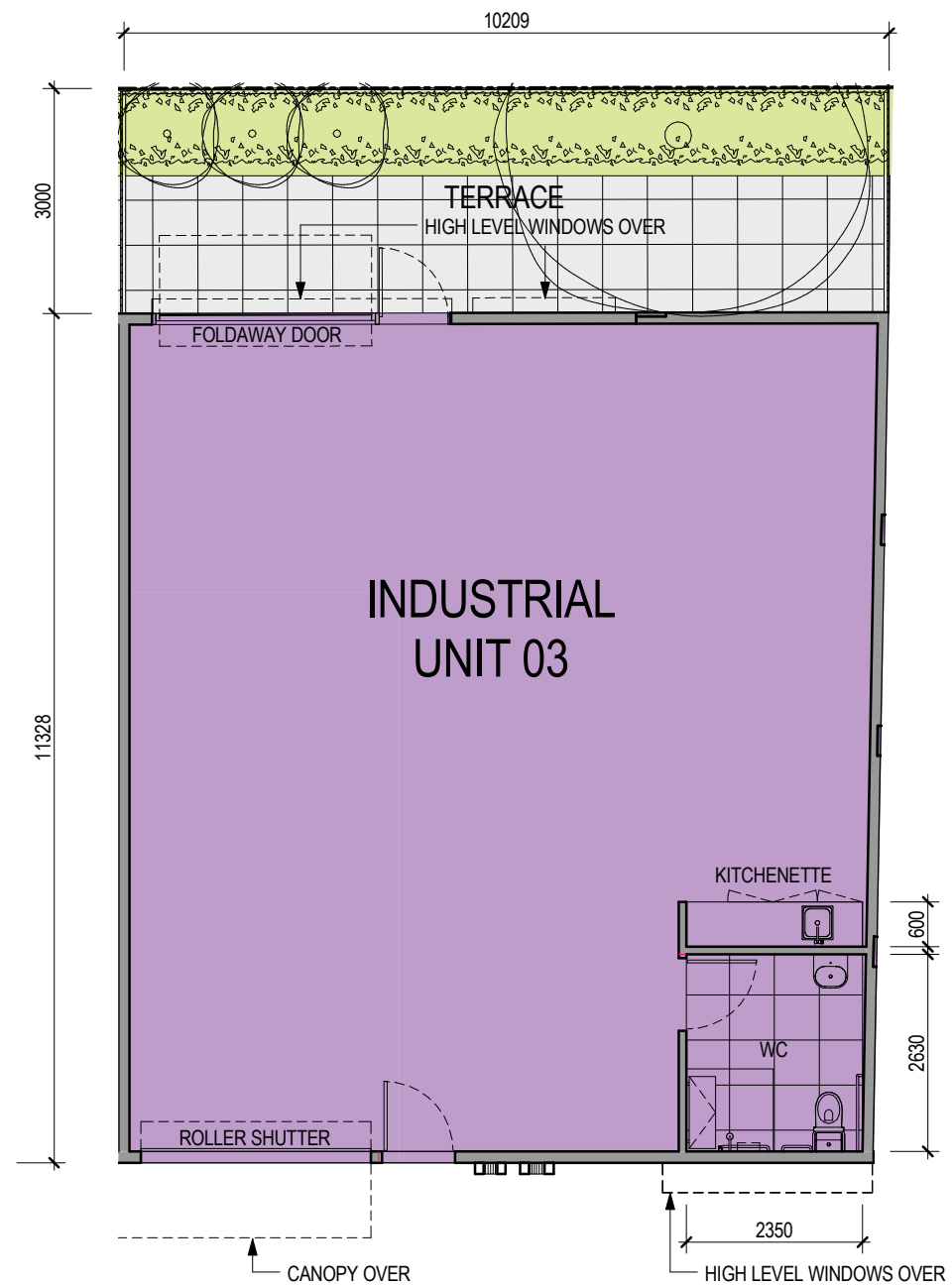
1 INDUSTRIAL UNIT 03 SCALE 1 : 100
