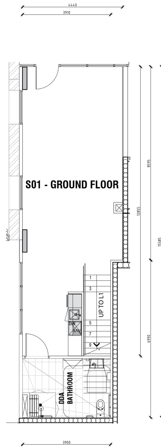
01 SO-01 OFFICE PLAN GROUND FLOOR
