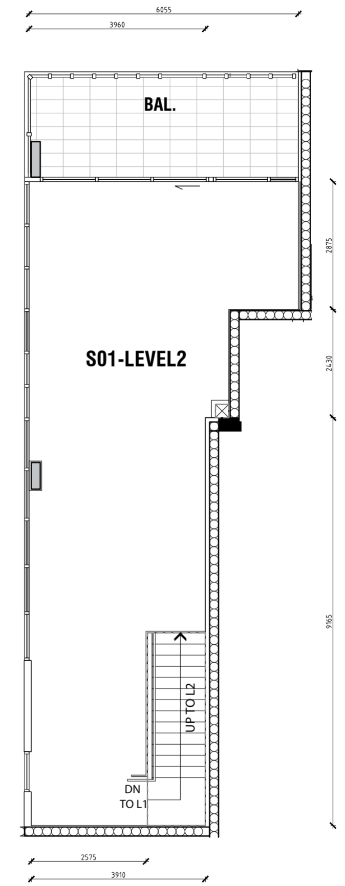
03 SO-01 OFFICE PLAN LEVEL 02
