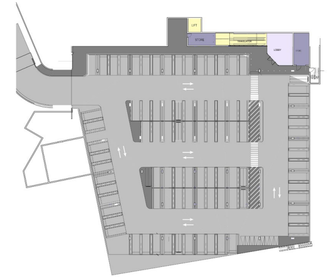
UNDERCROFT CARPARK PLAN
